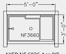
AKER NF 6036 AcrylX™ Alcove Shower Base 3' x 5' x 24" Integral Seat (ex. above)
