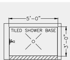
3' x 5' Tiled Shower Base or AKER ICON 6036 AcrylX™ Shower Base (ex. below)
